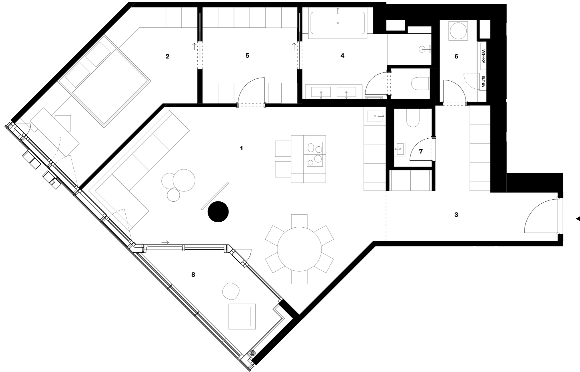
PLAN
